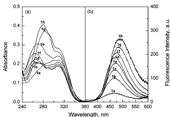
FIGURE 4. Absorption (a) and fluorescence (b) spectra of 1a–h in CH 3 CN.
