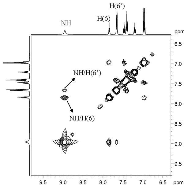
FIGURE 2. NOESY spectrum of 1d in CD 3 CN.
