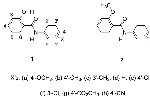
FIGURE 1. Chemical structures of salicylanilides 1a-h and methoxy counterparts 2a-g . 8a
