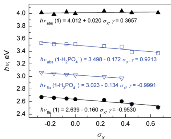
FIGURE 5. Linear correlation against the Hammett constant of substituent X of absorption and emission energies of 1 and its complex with H 2 PO 4 − in CH 3 CN. With 2 , the methoxy counterpart of 1 , h\nu_{\text{flu}} = 2.42 + 0.378\sigma_X . 8a
