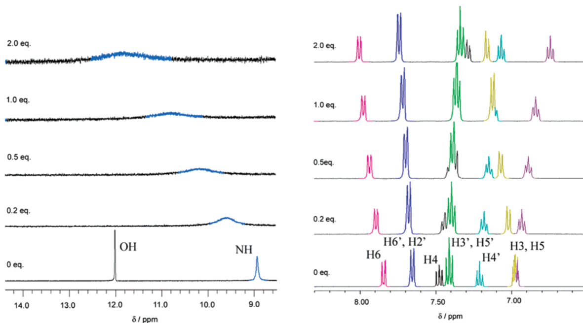
FIGURE 6. Portions of ^1\text{H} NMR spectra of 1d in \text{CD}_3\text{CN} in the presence of increasing equivalents of \text{H}_2\text{PO}_4^- as an n\text{-Bu}_4\text{N}^+ salt. [\mathbf{1d}] = 10 \text{ mmol L}^{-1} . For the numbering of the protons in 1d see Figure 1.
