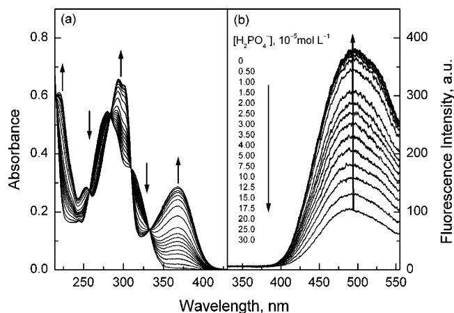
FIGURE 9. Absorption (a) and fluorescence (b) spectra of 1h ( X = p\text{-CN} ) in \text{CH}_3\text{CN} in the presence of increasing concentrations of \text{H}_2\text{PO}_4^- . [\mathbf{1h}] = 2.0 \times 10^{-5} (a) and 1.0 \times 10^{-5} (b) \text{mol L}^{-1} . The excitation wavelength employed to record the spectra in (b) was 283 nm, an isosbestic wavelength seen in (a).
