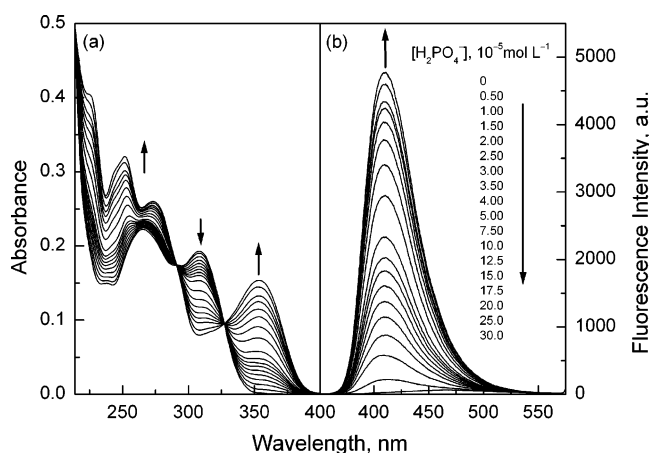
FIGURE 7. Absorption (a) and fluorescence (b) spectra of salicylanilide 1d in \text{CH}_3\text{CN} in the presence of increasing concentrations of \text{H}_2\text{PO}_4^- . [\mathbf{1d}] = 2.0 \times 10^{-5} (a) and 1.0 \times 10^{-5} (b) \text{mol L}^{-1} . The excitation wavelength employed to record the spectra in (b) was 290 nm, an isosbestic wavelength seen in (a).
