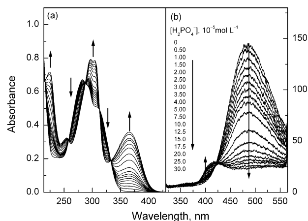
FIGURE 8. Absorption (a) and fluorescence (b) spectra of 1g ( X = p\text{-CO}_2\text{CH}_3 ) in \text{CH}_3\text{CN} in the presence of increasing concentrations of \text{H}_2\text{PO}_4^- . [\mathbf{1g}] = 3.5 \times 10^{-5} (a) and 1.8 \times 10^{-5} (b) \text{mol L}^{-1} . The excitation wavelength employed to record the spectra in (b) was 287 nm, an isosbestic wavelength seen in (a).
