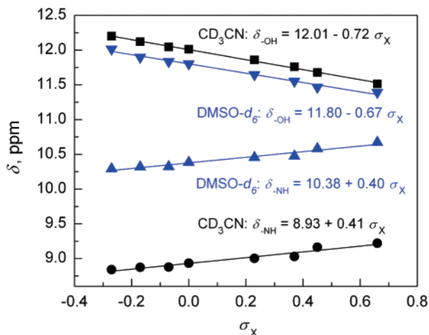
FIGURE 3. Linear relationship against the Hammett constant of substituent X in 1a–h of the chemical shifts of the OH and NH protons in CD 3 CN and DMSO- d 6 . With 2 , the methoxy counterpart of 1 , in DMSO- d 6 , \delta(\text{NH}) = 10.12 + 0.61\sigma_X . 8a
