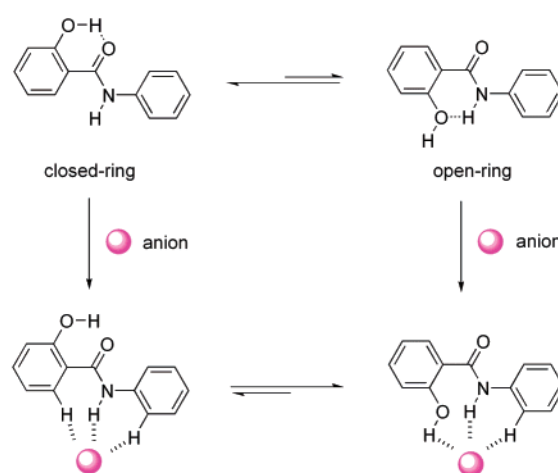
SCHEME 2. Conformational Equilibria of 1d in the Presence of H 2 PO 4 −
